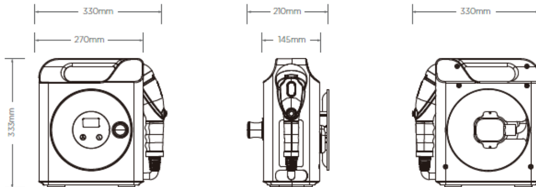
Charger Dimensions:
